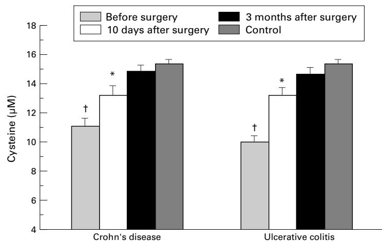
Figure 2 Fasting plasma cysteine levels in patients with Crohn's disease ( n=33 ) and ulcerative colitis ( n=33 ) before surgery and 10 days and three months after complete resection of inflamed bowel. Bars represent mean (SE). Data were statistically analysed by the Student's t test for unpaired samples including a Bonferroni's correction. * p<0.008 , † p<10^{-4} versus controls ( n=65 ).
