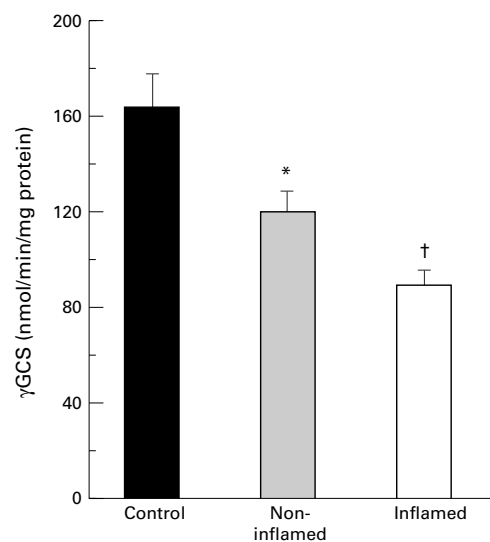
Figure 6 Decreased mucosal enzyme activity of gamma-glutamylcysteine synthetase (gammaGCS) in inflamed ( n=26 ) and non-inflamed ( n=21 ) ileum of patients with Crohn's disease. Bars represent mean (SE). Statistical analysis was performed by the Student's t test for unpaired samples including a Bonferroni's correction. * p<0.025 , † p<10^{-4} versus controls ( n=21 ).
