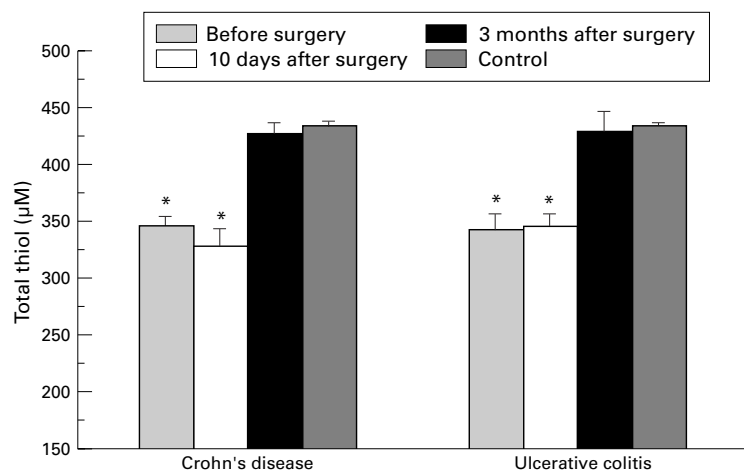
Figure 4 Total thiol levels in non-deproteinised plasma in patients with Crohn's disease ( n=33 ) and ulcerative colitis ( n=33 ) before surgery and 10 days and three months after complete resection of inflamed bowel. Values represent means (SE) and were statistically analysed by the Student's t test for unpaired samples. According to Bonferroni's correction the level of significance was set at p<0.008 . * p<10^{-4} versus controls ( n=65 ).
